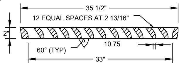
SECTION C-C
