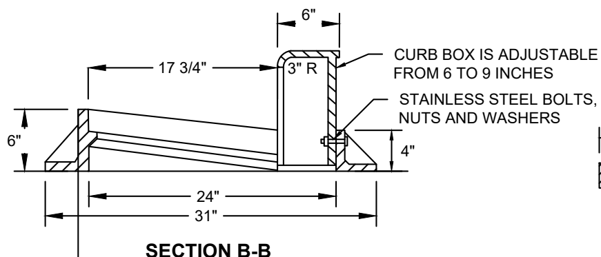
SECTION B-B
